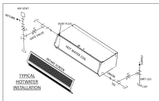
FIG. 3 (Hot Water Heated STD2 Unit)
