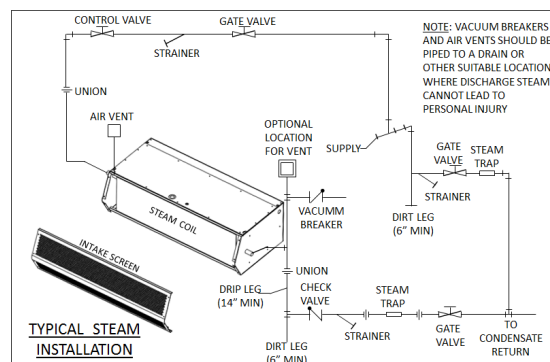
FIG. 4 (Steam Heated STD2 Unit)
