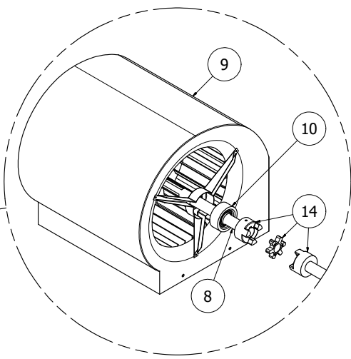
DETAIL 4
