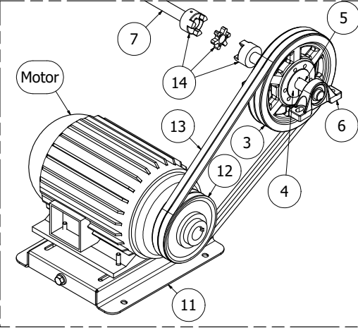
DETAIL 1
