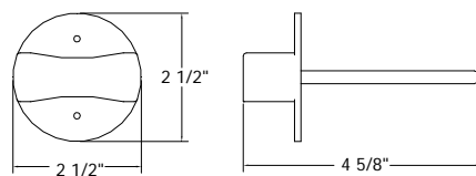
99-187 – Duct Air Temperature Sensor, 24 Volt, 10k Ohms
