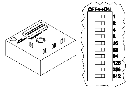
INS-TD: Adjustable Time Delay (Turn ON dip switches to add time delay)
